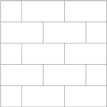
Broken Bond Stripping optional Tile sizes: 304.8 x 457.2 mm 304.8 x 609.6 mm 457.2 x 914.4 mm
