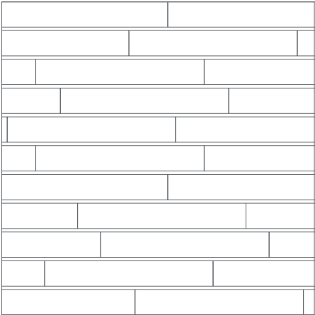
Deck Block Stripping required Plank sizes: 76.2 x 914.4 mm 114.3 x 914.4 mm 152.4 x 914.4 mm 184.2 x 1219.2 mm
