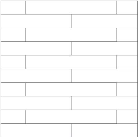
Linear Block Stripping optional Tile sizes: 76.2 x 914.4 mm 114.3 x 914.4 mm 152.4 x 914.4 mm
