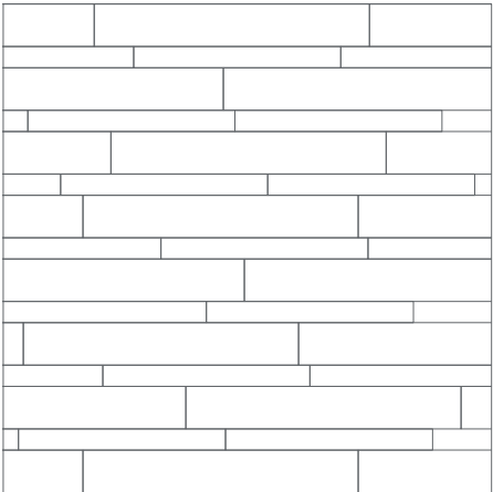
Boardwalk Plank sizes: 76.2 x 914.4 mm 114.3 x 914.4 mm 152.4 x 914.4 mm
